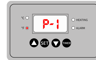
P-1: Temp. Setting Mode Touch SET & ▲▼ to set desired Temp.
